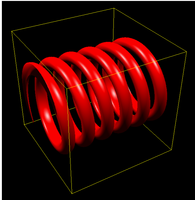
FIG. 8. Replication of two subsets of pieces of a mechanical spring
