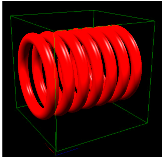
FIG. 7. Example of a torus replication
