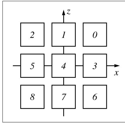
FIG. 3. Nine cases for determining \Theta bounds
