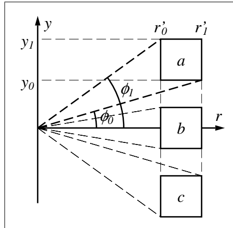
FIG. 5. Three cases for determining \Phi bounds
