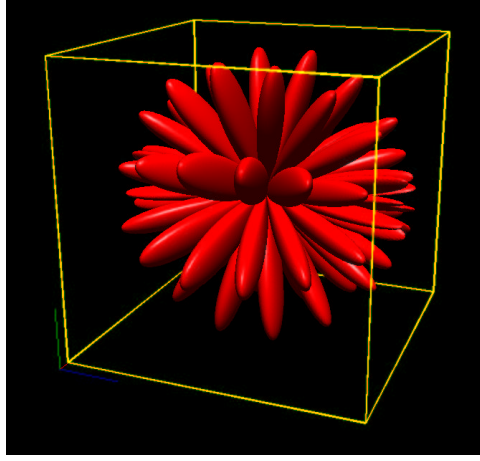
FIG. 13. \sin(4\theta) \cdot \sin(8\phi) - R = 0
