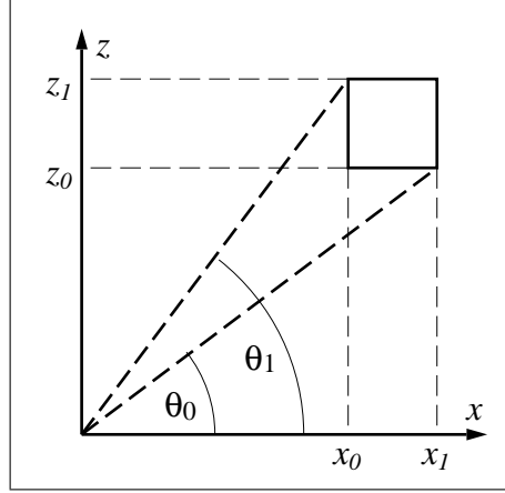
FIG. 4. Determining \Theta bounds for case 0
