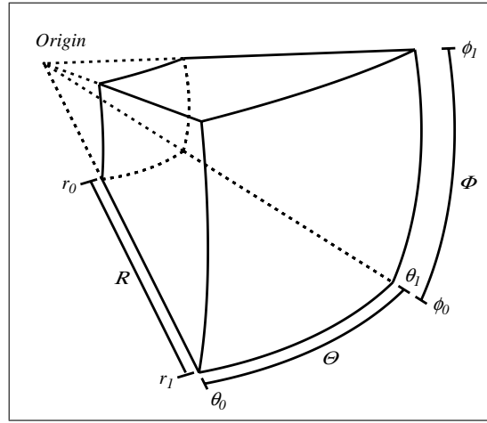
FIG. 2. Intervals \mathbf{R}[r_0, r_1] , \mathbf{\Theta}[\theta_0, \theta_1] and \mathbf{\Phi}[\phi_0, \phi_1]
